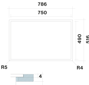
Flush installation
